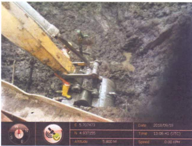
Figure 1: Exposing the pipeline.
